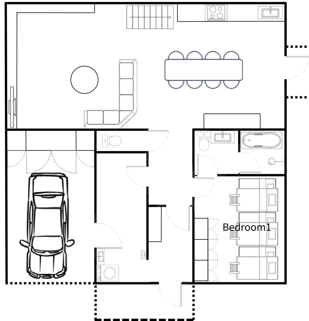
1st Floor
