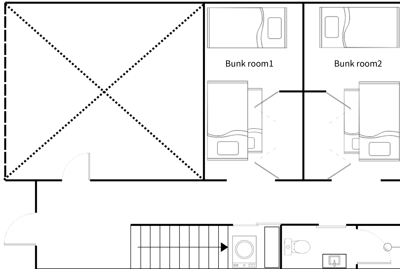
1st Floor
